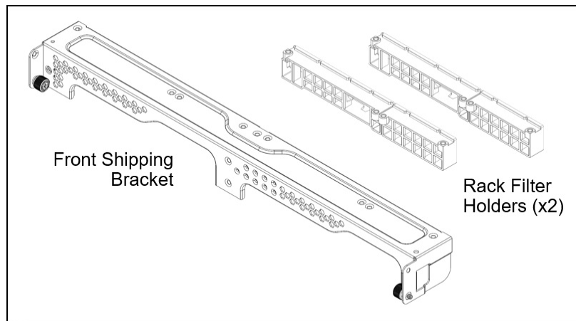
Figure 28. ThinkSystem Enclosure Front Shipping Bracket
